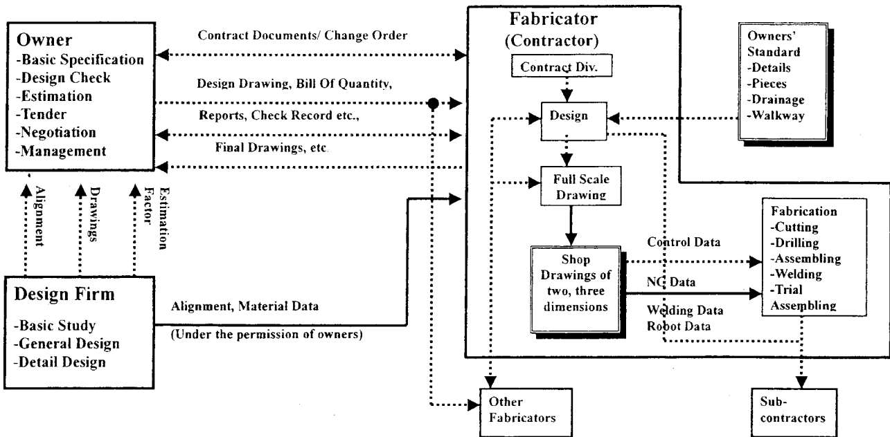
Fig. 1 Conventional data exchange in the construction work of steel bridge superstructure
