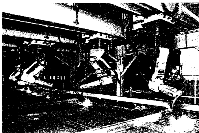
Fig. 7 Welding robots with multi-joints in bridge factory
