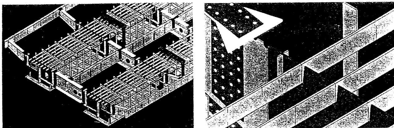
Fig. 8 The bird's-eye view and the details of RC box girder by solid model
